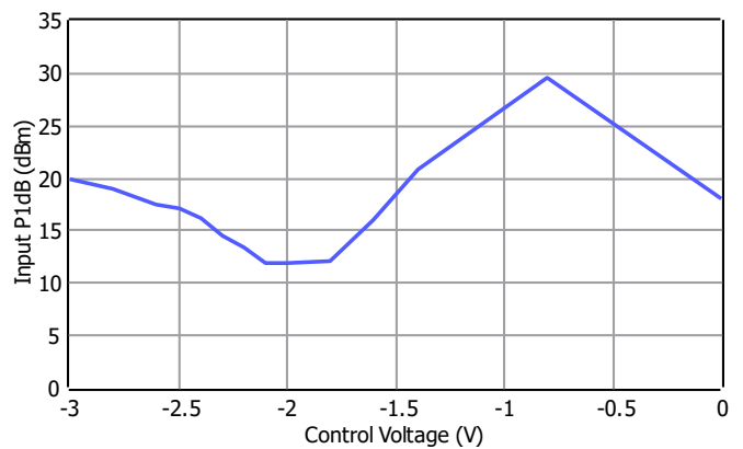
Input P1dB vs Control Voltage at 10 GHz
