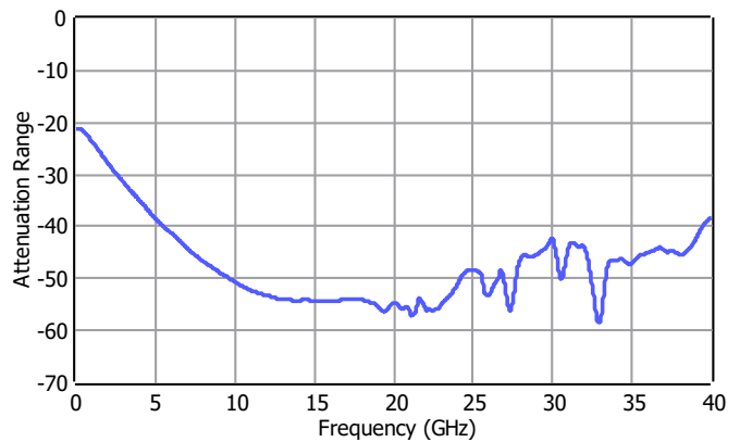
Attenuation Range
